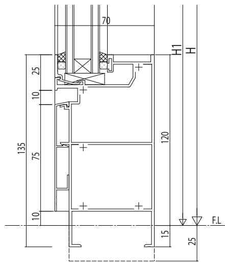
135mm見付幅木
