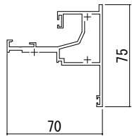
●FIX窓/可動窓
