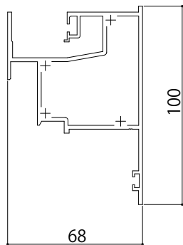
■外倒し・突出し【排煙窓・隠ぺい】／FIX(38mm) ■FIX(18・28mm)／可動 [2K-84487]
