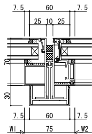
●FIX窓/可動窓
