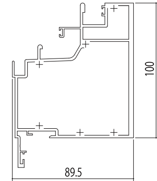
■引違い(4枚建)・両袖片引き／FIX(内押縁) [2K-64431]
