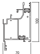
■引違い・片引き/ FIX(内押縁)[2BK-61082]
