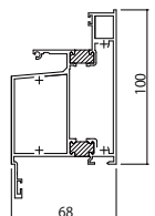
■可動/FIX[2BK-61090]
