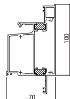
■可動/可動[2BK-61091]
