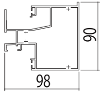
●FIX/FIX(23・33mm) [2K-75381]
