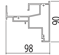
●FIX(38・48mm)/たてすべり出し [2K-75382]
