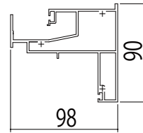
●FIX(23・33mm)/大型たてすべり出し [2K-75388]
