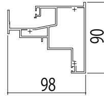
●FIX(23・33mm)/たてすべり出し [2K-75383]
