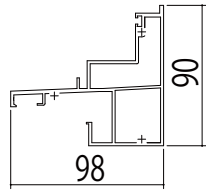
●可動/FIX(38・48mm) [2K-75384]
