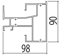
●FIX/FIX(38・48mm) [2K-75380]
