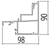
●可動/FIX(23・33mm) [2K-75385]
