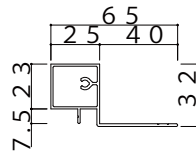
縦見切縁K-88291
