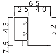
縦見切縁K-88294
