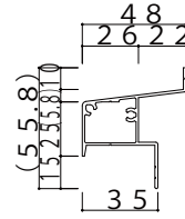
下見切縁K-88289
