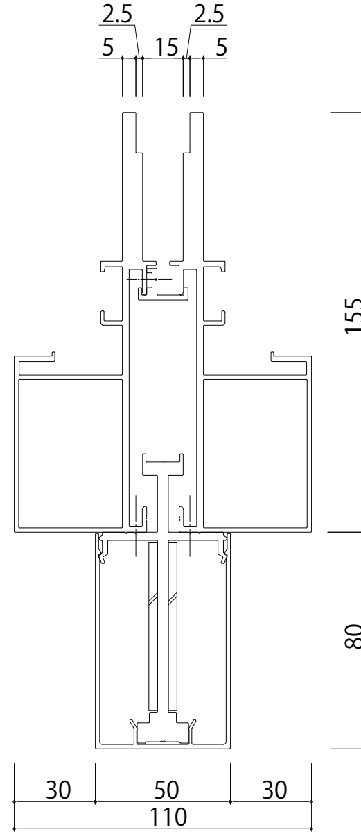
●A方立[K-99497]
