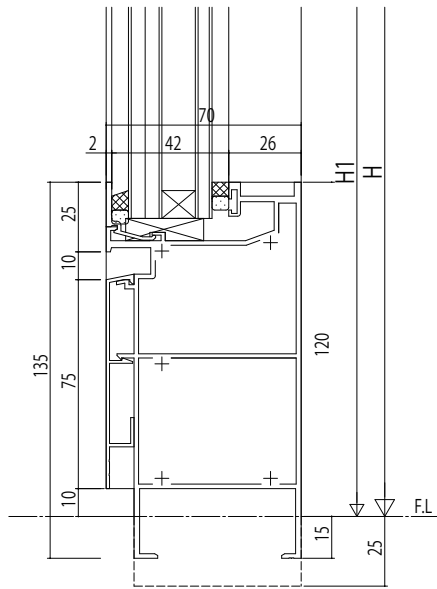
135mm見付幅木
