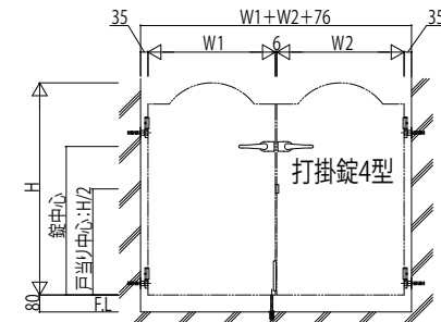
埋込金具式内開き外観姿図(1:10)
