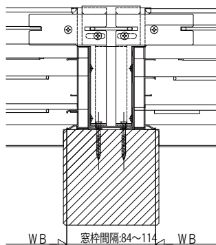
WB 窓枠間隔:84~114 WB
