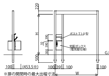
姿図(1:10)
