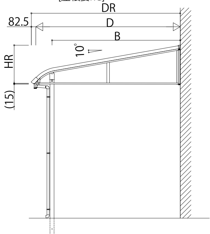
[屋根妻RG]
