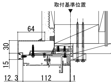
●外額縁 (21)
