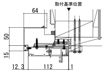
●外額縁 (50)
