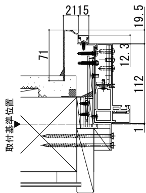
●外額縁 (80K)
